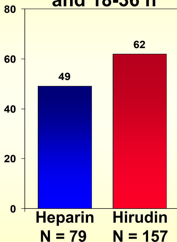
TIMI 3 Flow at 90' and 18-36 h
