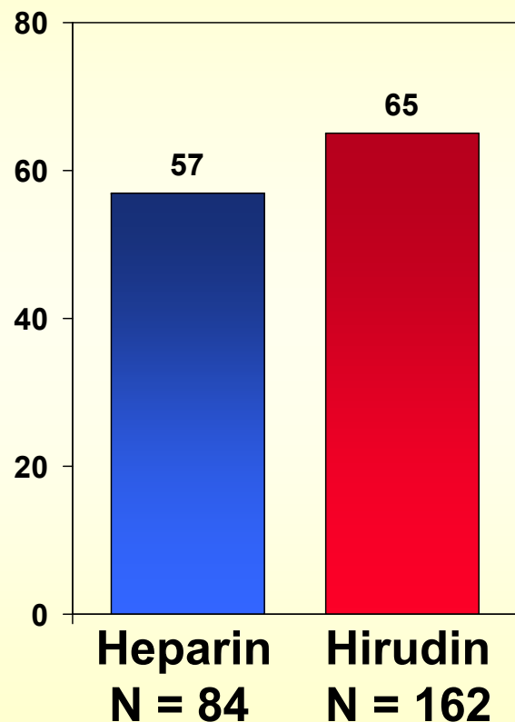
TIMI 3 Flow at 90'
